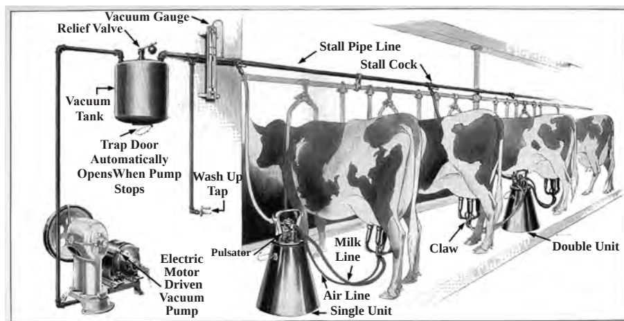
Milking Machine
