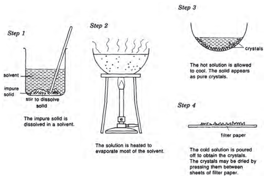
Fig.4: Crystallization
